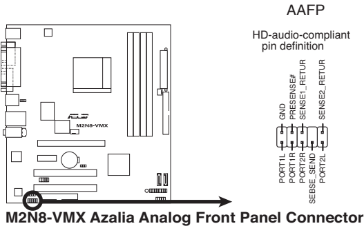
M2N8-VMX Azalia Analog Front Panel Connector
